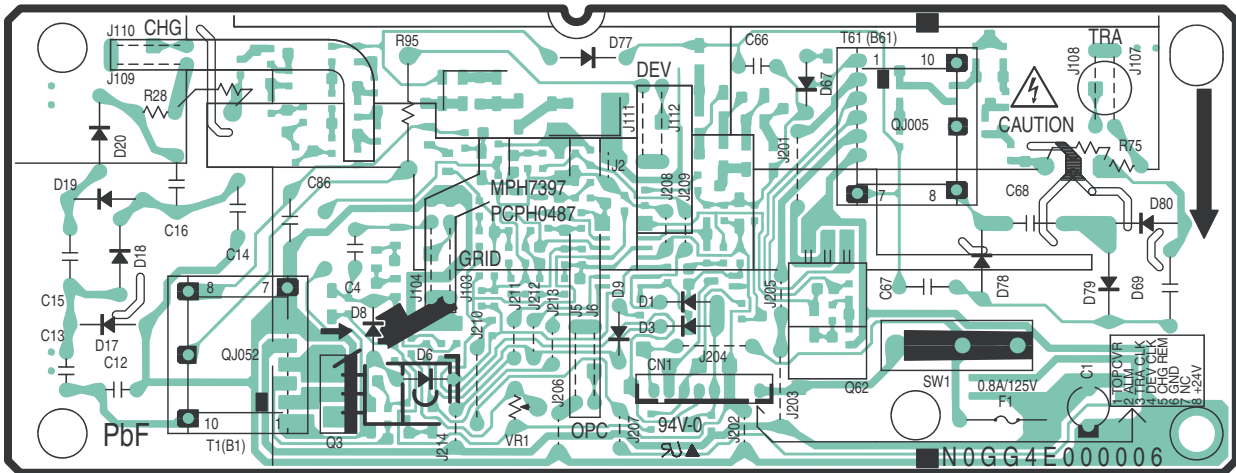
KX-MB2230EU / KX-MB2270EU / KX-MB2515EU / KX-MB2545EU / KX-MB2575EU / DP-MB310EU HIGH VOLTAGE POWER SUPPLY BOARD (COMPONENT VIEW)
