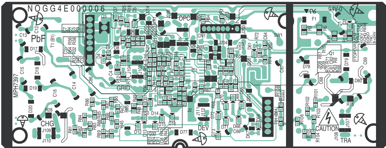
KX-MB2230EU / KX-MB2270EU / KX-MB2515EU / KX-MB2545EU / KX-MB2575EU / DP-MB310EU HIGH VOLTAGE POWER SUPPLY BOARD (BOTTOM VIEW)
