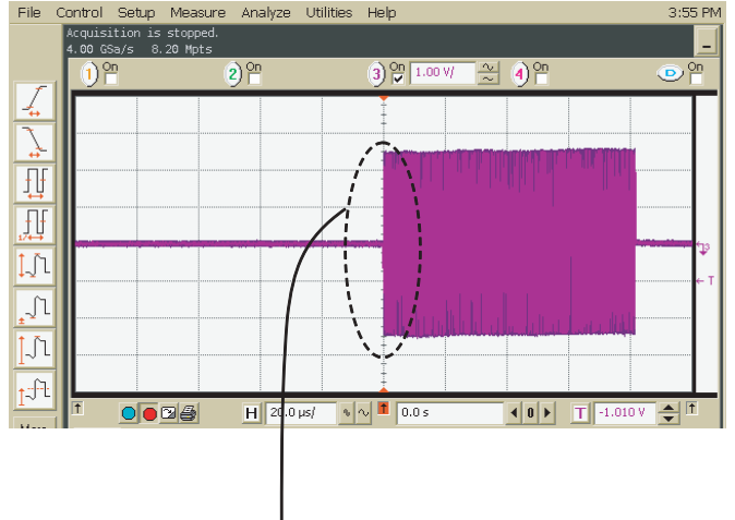
③ 10Base-T waveform 3 [ during data commnication ]
