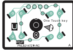
DP-MB310EU ONE TOUCH KEY BOARD
