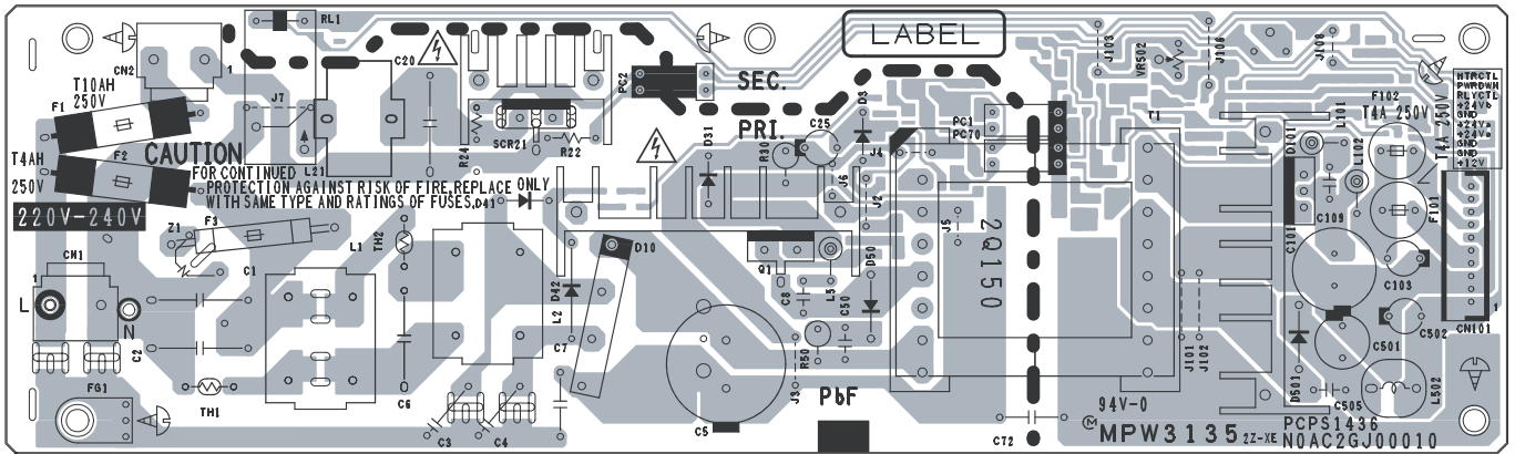
KX-MB2230EU / KX-MB2270EU / KX-MB2515EU / KX-MB2545EU / KX-MB2575EU / DP-MB310EU LOW VOLTAGE POWER SUPPLY BOARD (COMPONENT VIEW)
