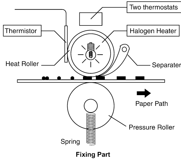
Fixing Part
