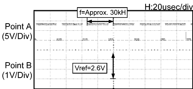
(1) Full speed mode Duty=80.0%
