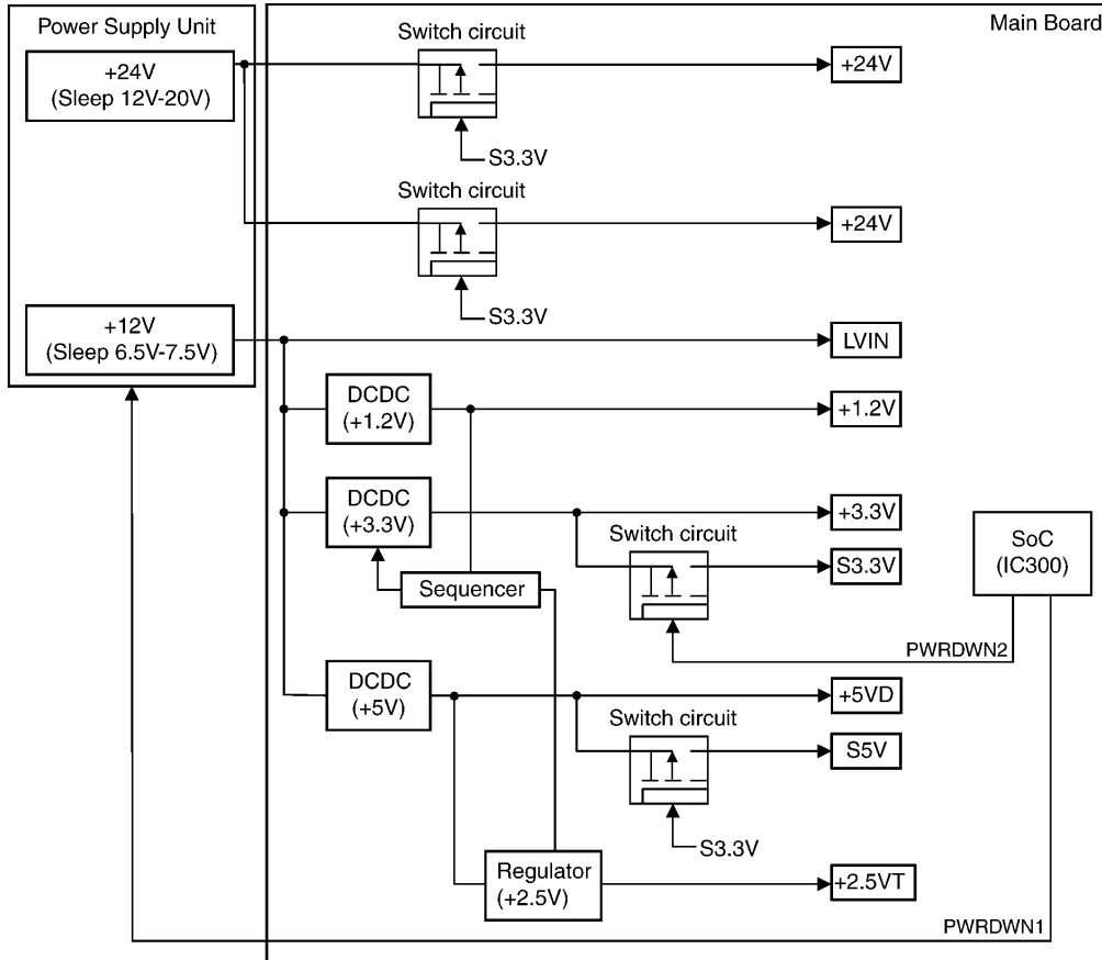
Sleep Control Flow
