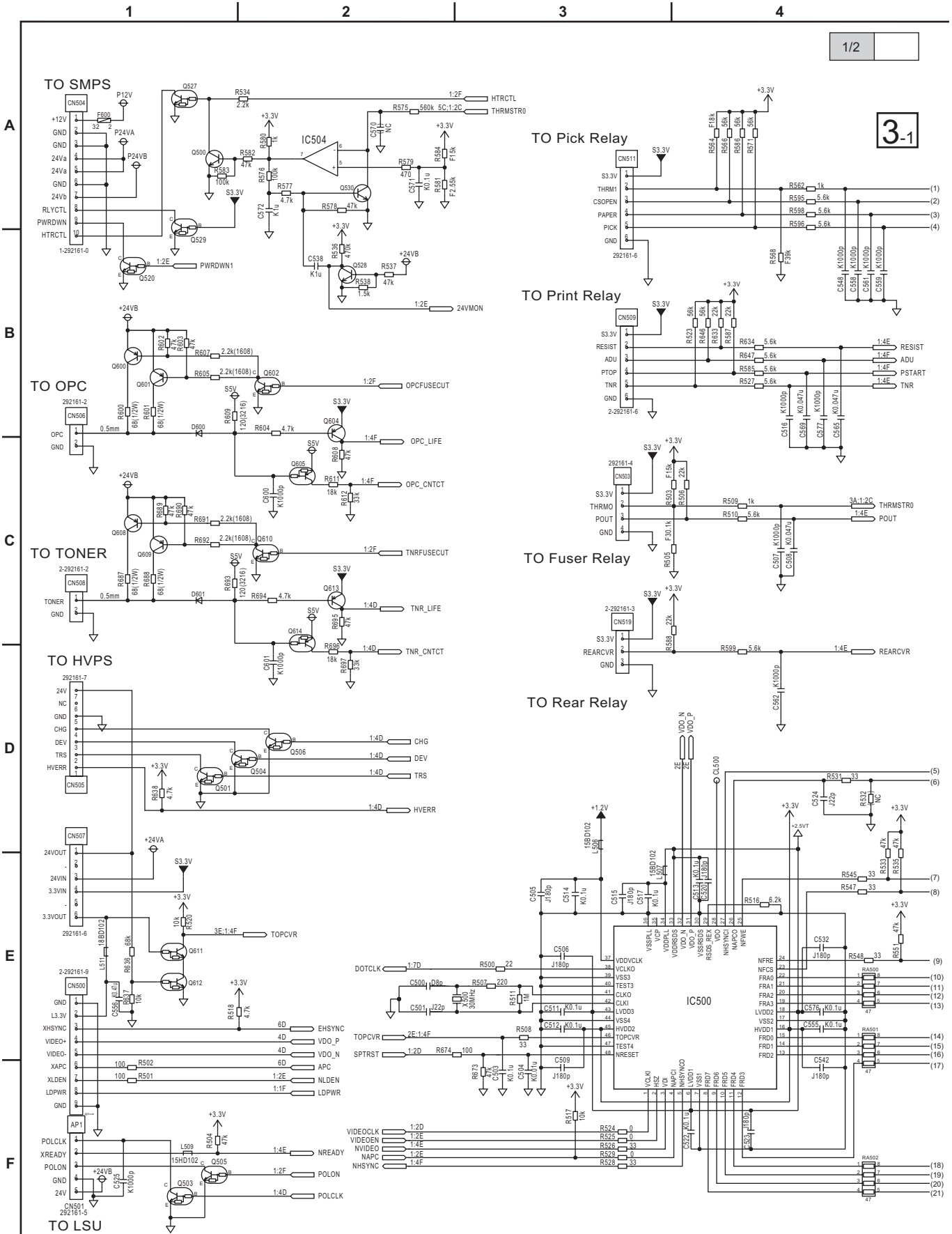
KX-MB2575EU MAIN BOARD (No.3) (1/2)
