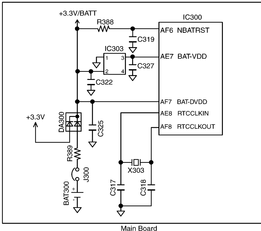
Circuit Diagram
