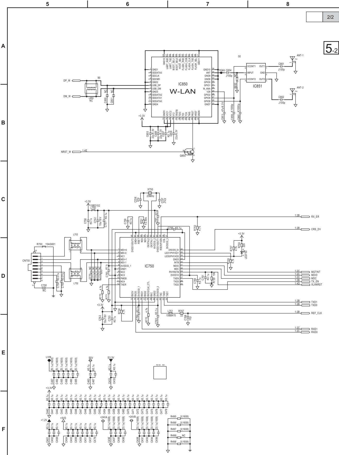
KX-MB2575EU MAIN BOARD (No.5) (2/2)
