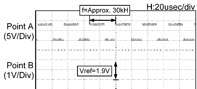
(2) Half speed mode Duty=56.6%
