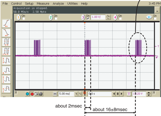
① Auto negotiation waveform 1
